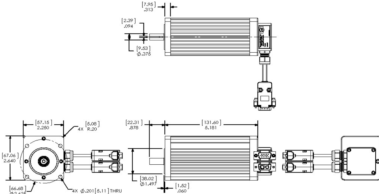
Figure 1 – Outline Drawing
